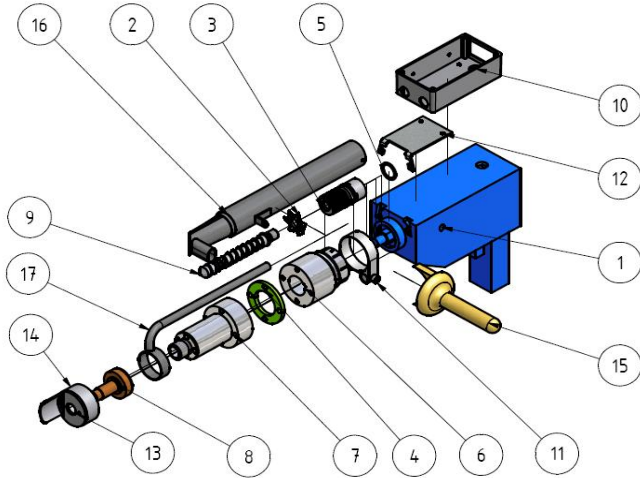
20440 EXWELD sigma EC
